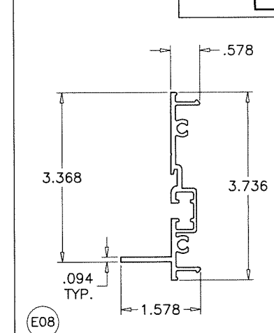
E08 DOOR MULL SNAP-IN MATE
