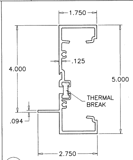
E04M VERTICAL MULLION
