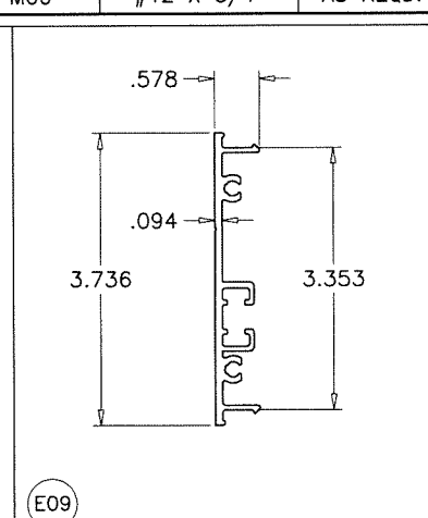
E09 DOOR MULL SNAP-IN PLATE
