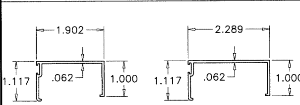
E05 GLAZING BEADS
